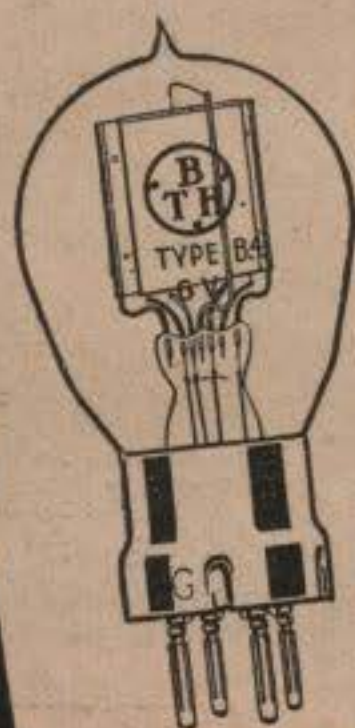
B4 Type Filament Volts - 6 volts Filament Current - 0.25 amps Anode Volts - 40-100 volts
