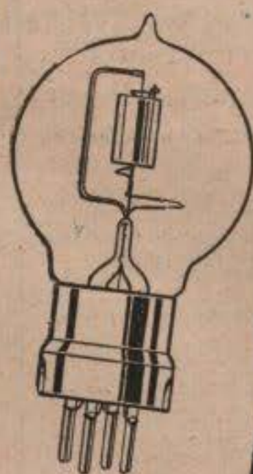
R Type Filament Volts - 4 volts Filament Current - 0.67 amps Anode Volts - 40-60 volts
